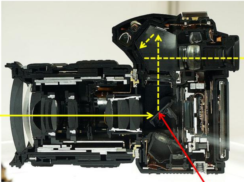
Reflex mirror is down
