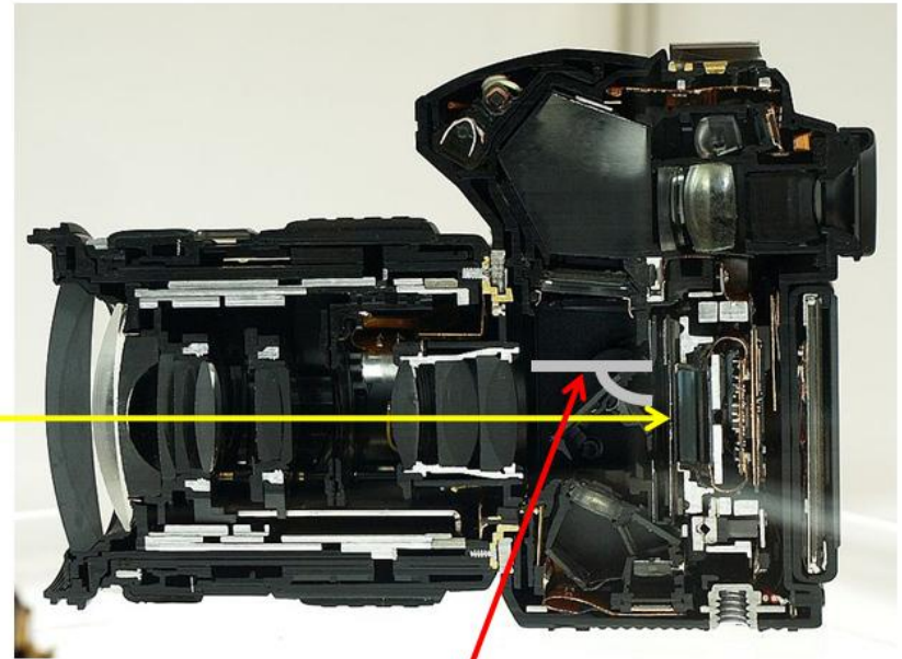
Reflex mirror is up, exposing image sensor
